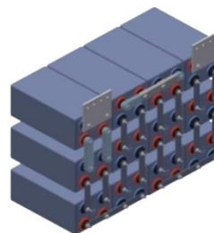
Fig. 10 Image of horizontal installation
