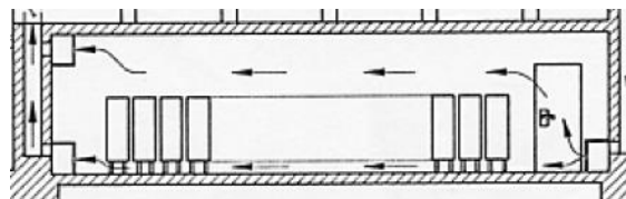
Fig. 13 Opening on opposite walls
