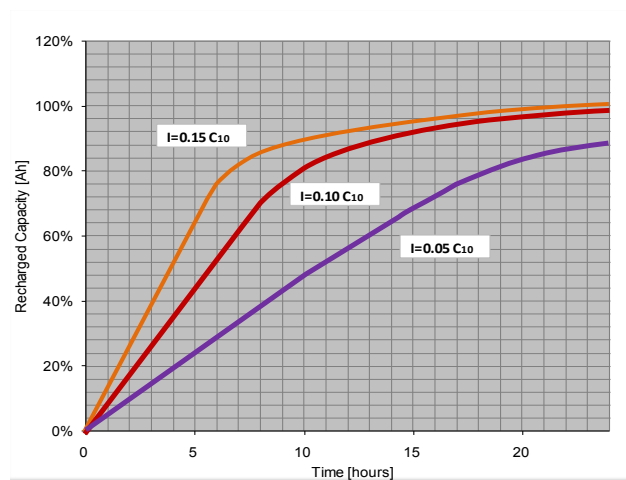
Fig. 7 Recharge curves at 2.4 volt per cell with different limit of current
