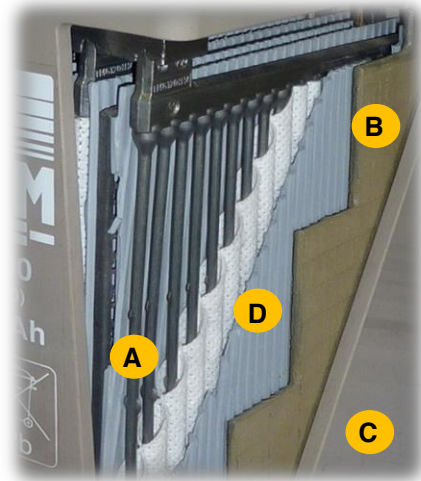
Cutaway drawing of FIAMM GEL cell
