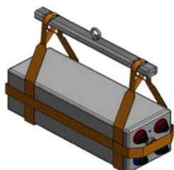
Fig. 8 Image of strap for horizontal handling.
