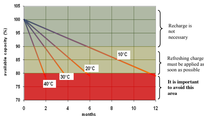
Fig. 12 Storage time versus temperatures.
