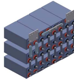
Example of installation and cell arrangement (position of + / - poles) of AGM batteries with capacity equal or higher than 800Ah
